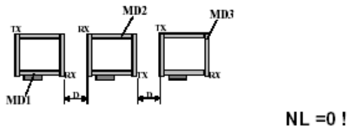
Fig. 11 Installation of 3 Metal Detectors ( D \geq 20\text{cm} ).
