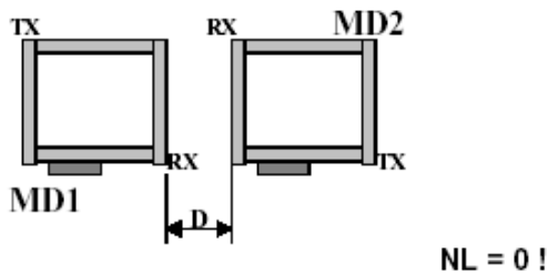
Fig. 10 Installation of 2 Metal Detectors ( D \geq 5\text{cm} ).
